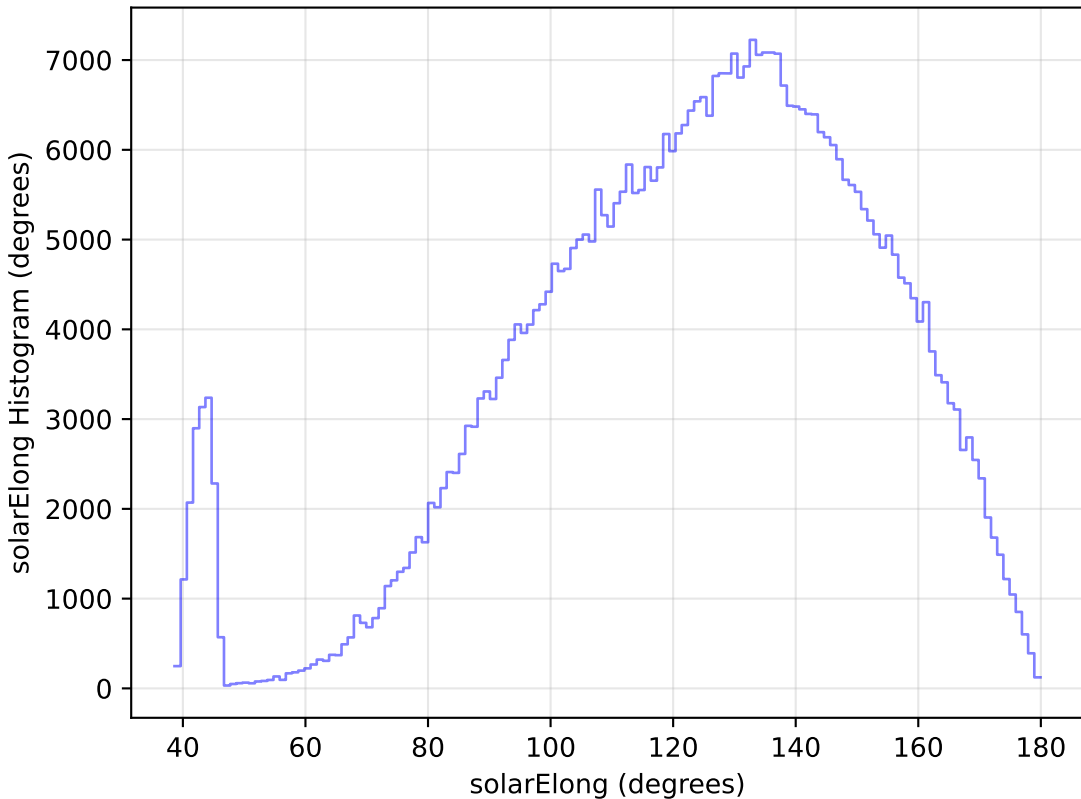
too_5_1v3.4_10yrs WFD r band: solarElong Histogram
