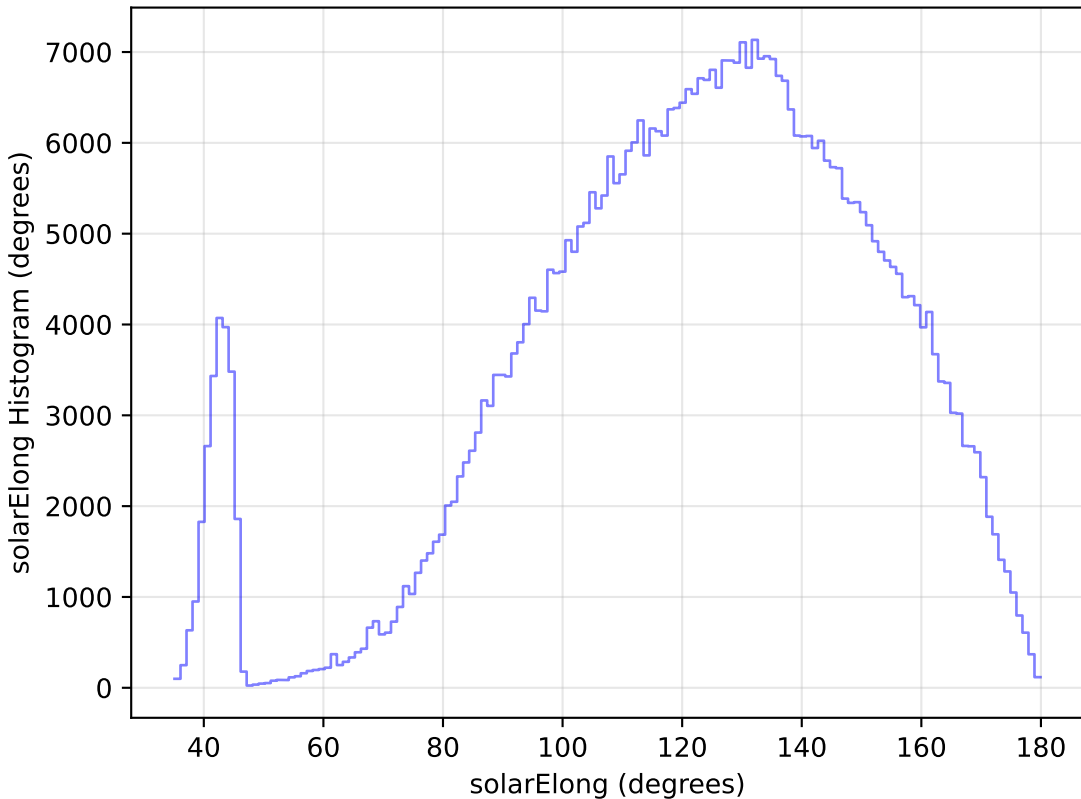
too_5_1v3.4_10yrs WFD i band: solarElong Histogram
