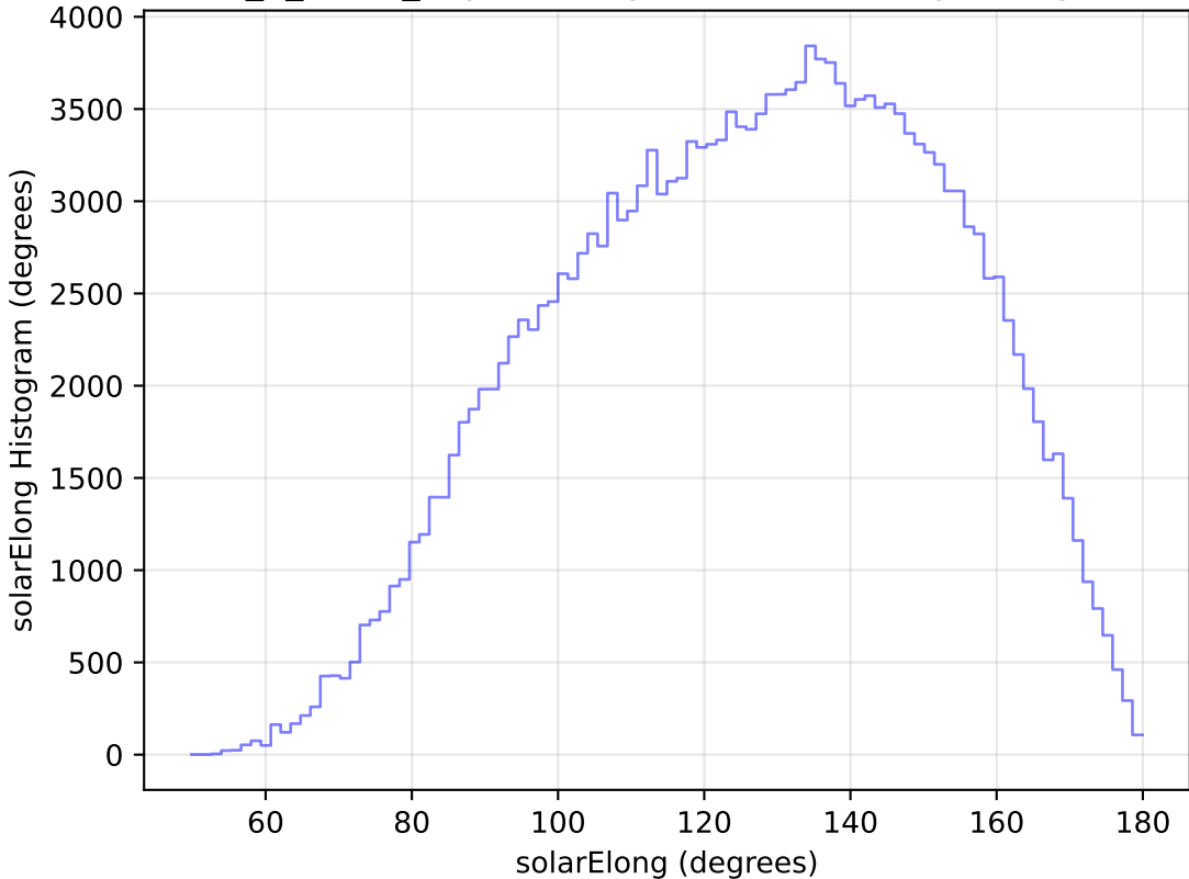
too_5_1v3.4_10yrs WFD g band: solarElong Histogram
