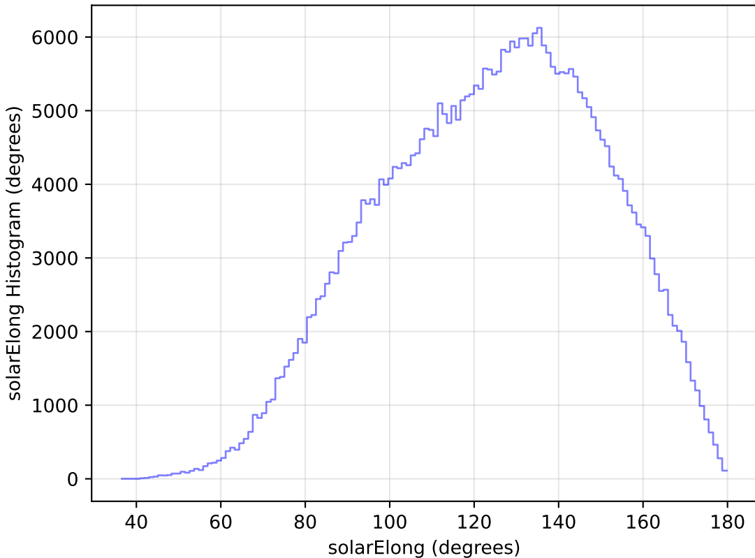
too_5_1v3.4_10yrs All sky y band: solarElong Histogram
