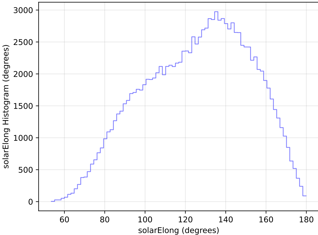
too_5_1v3.4_10yrs All sky u band: solarElong Histogram
