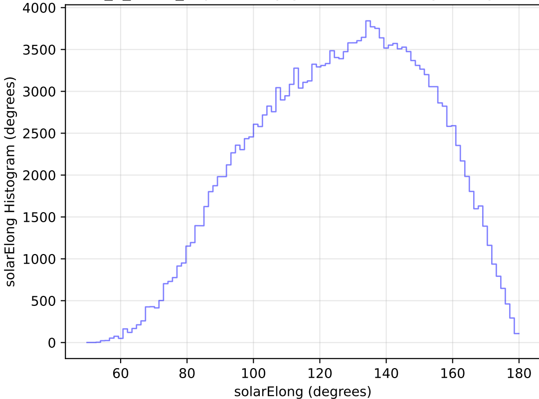
too_5_1v3.4_10yrs All sky g band: solarElong Histogram
