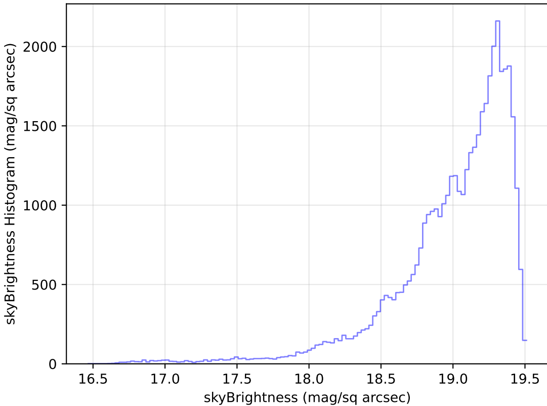
too_5_1v3.4_10yrs Yr 1 z band: skyBrightness Histogram
