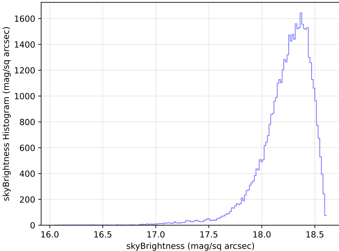
too_5_1v3.4_10yrs Yr 1 y band: skyBrightness Histogram
