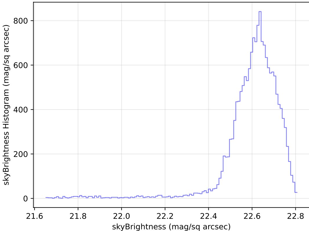
too_5_1v3.4_10yrs Yr 1 u band: skyBrightness Histogram
