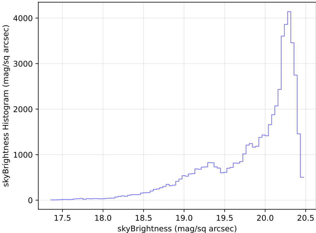
too_5_1v3.4_10yrs Yr 1 i band: skyBrightness Histogram
