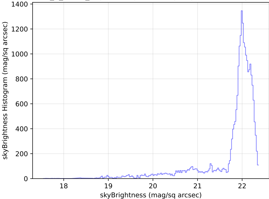
too_5_1v3.4_10yrs Yr 1 g band: skyBrightness Histogram
