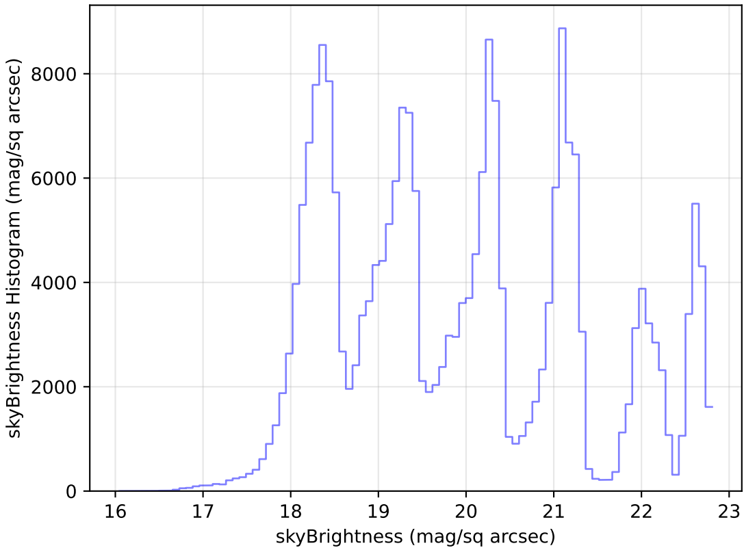
too_5_1v3.4_10yrs Yr 1 all bands: skyBrightness Histogram
