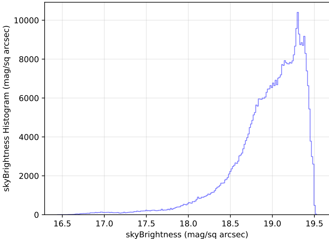
too_5_1v3.4_10yrs WFD z band: skyBrightness Histogram
