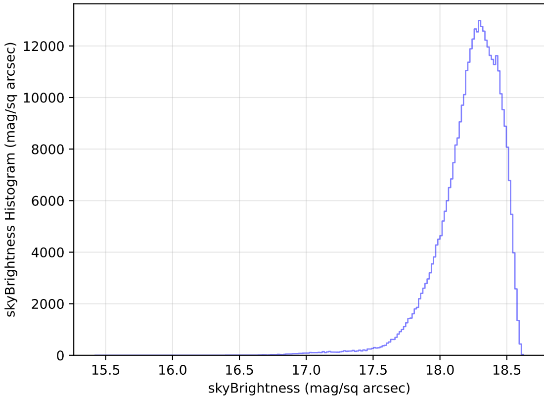
too_5_1v3.4_10yrs WFD y band: skyBrightness Histogram
