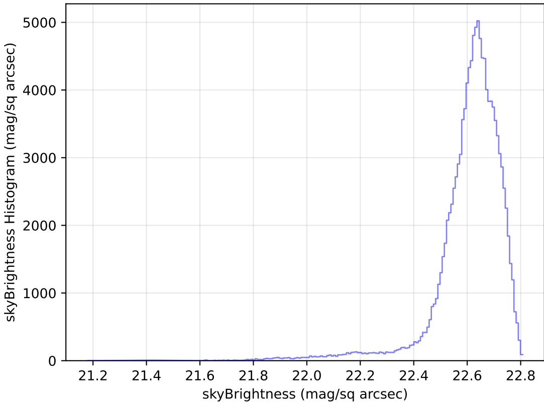
too_5_1v3.4_10yrs WFD u band: skyBrightness Histogram
