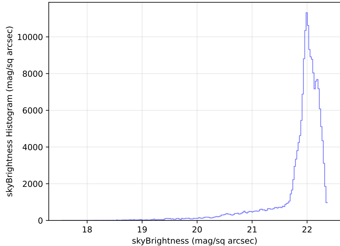
too_5_1v3.4_10yrs WFD g band: skyBrightness Histogram
