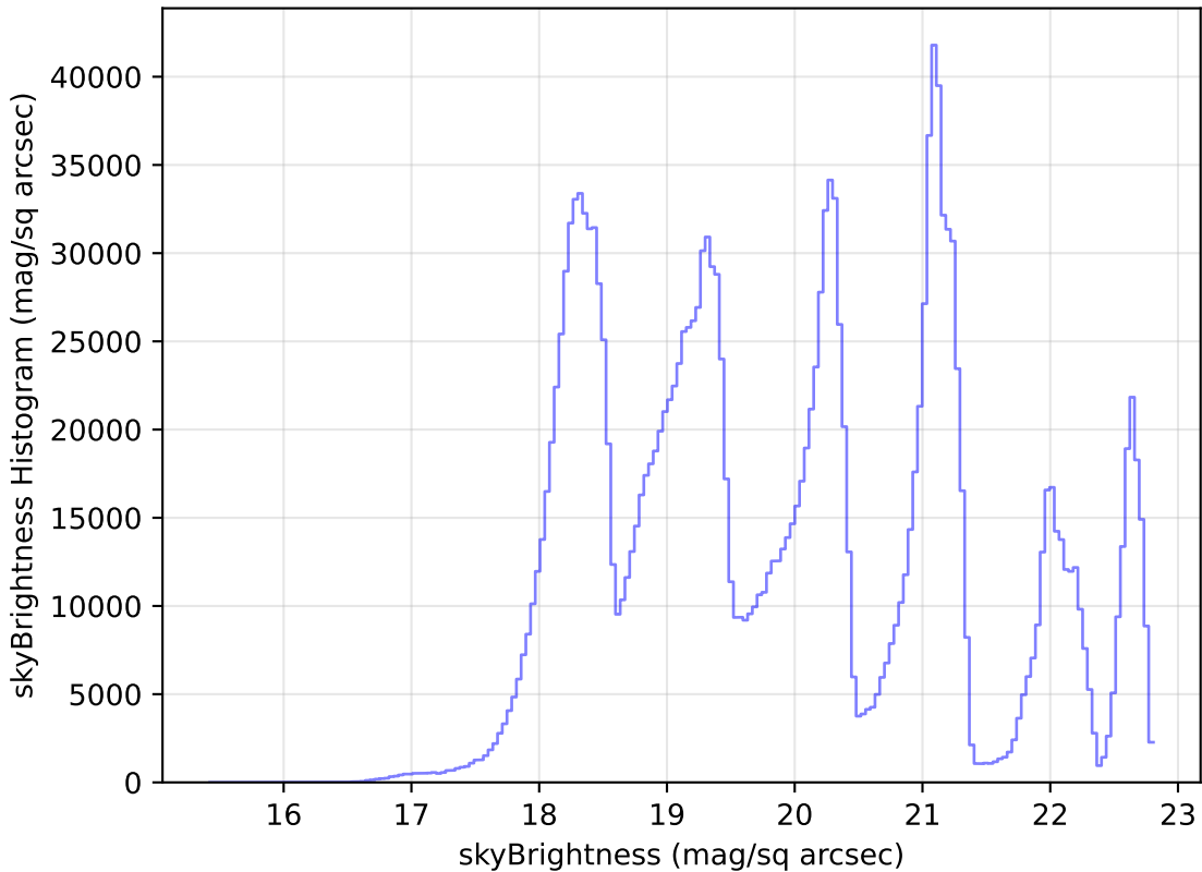
too_5_1v3.4_10yrs WFD all bands: skyBrightness Histogram
