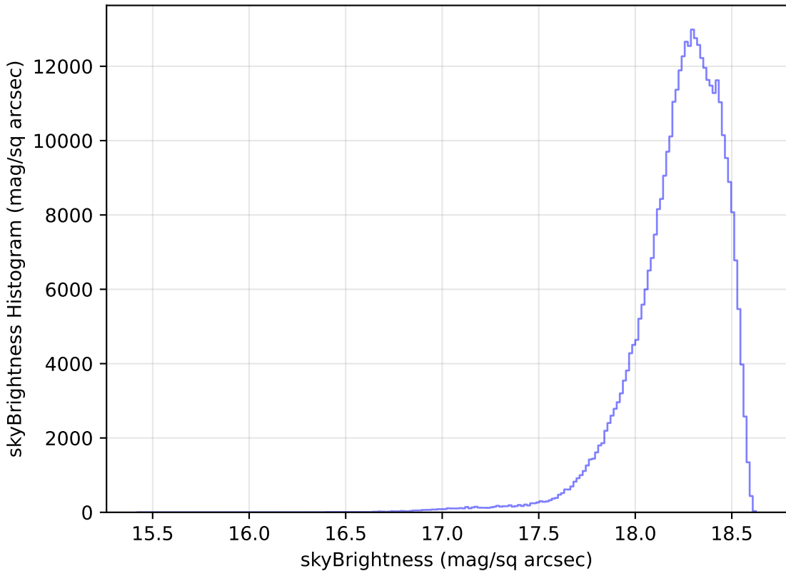
too_5_1v3.4_10yrs All sky y band: skyBrightness Histogram
