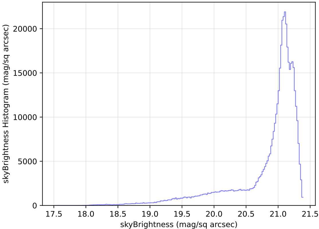
too_5_1v3.4_10yrs All sky r band: skyBrightness Histogram
