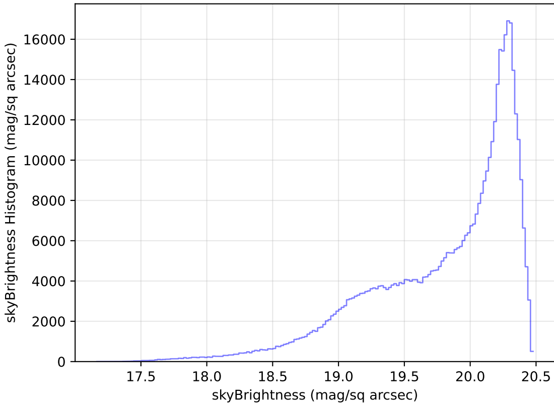
too_5_1v3.4_10yrs All sky i band: skyBrightness Histogram
