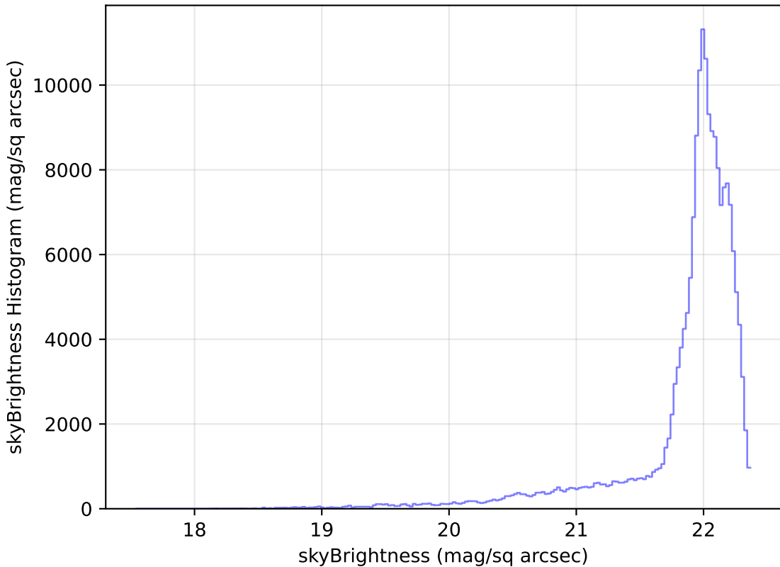
too_5_1v3.4_10yrs All sky g band: skyBrightness Histogram
