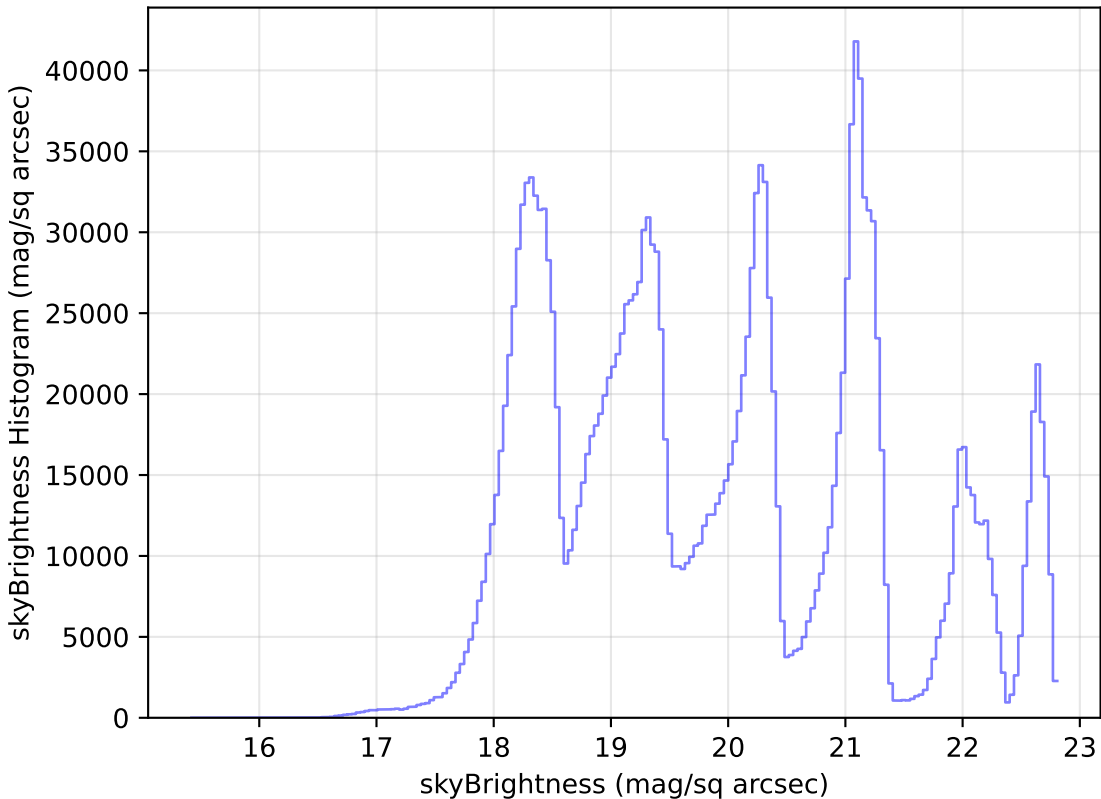
too_5_1v3.4_10yrs All sky all bands: skyBrightness Histogram
