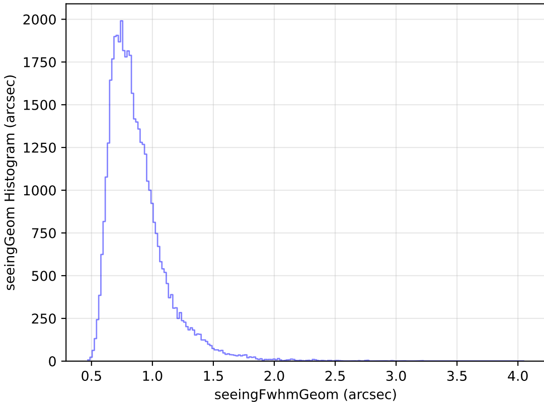
too_5_1v3.4_10yrs Yr 1 z band: seeingGeom Histogram
