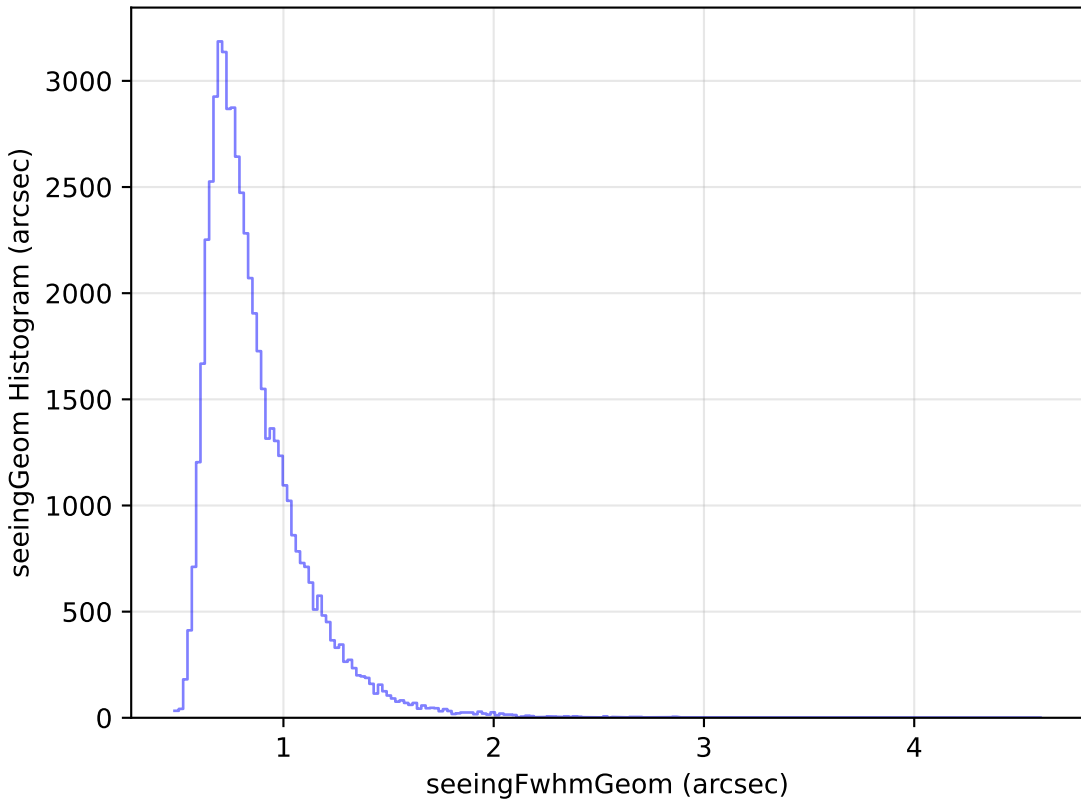
too_5_1v3.4_10yrs Yr 1 i band: seeingGeom Histogram
