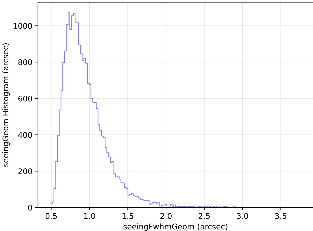
too_5_1v3.4_10yrs Yr 1 g band: seeingGeom Histogram
