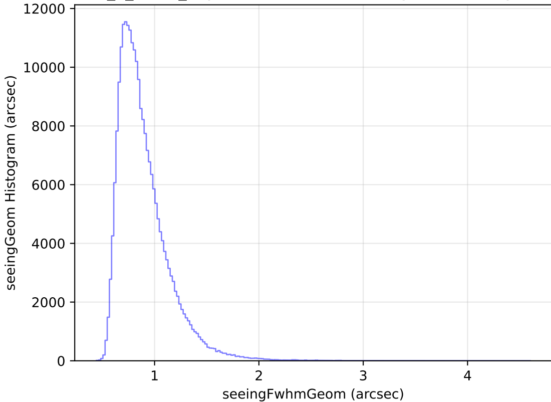
too_5_1v3.4_10yrs Yr 1 all bands: seeingGeom Histogram
