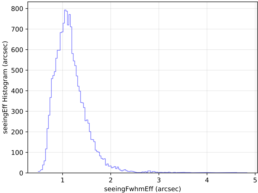
too_5_1v3.4_10yrs Yr 1 u band: seeingEff Histogram
