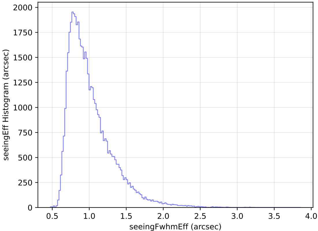
too_5_1v3.4_10yrs Yr 1 r band: seeingEff Histogram
