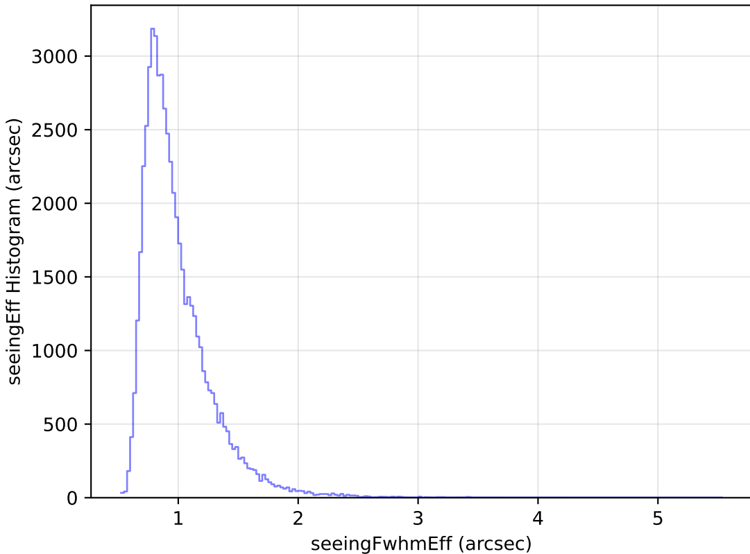
too_5_1v3.4_10yrs Yr 1 i band: seeingEff Histogram
