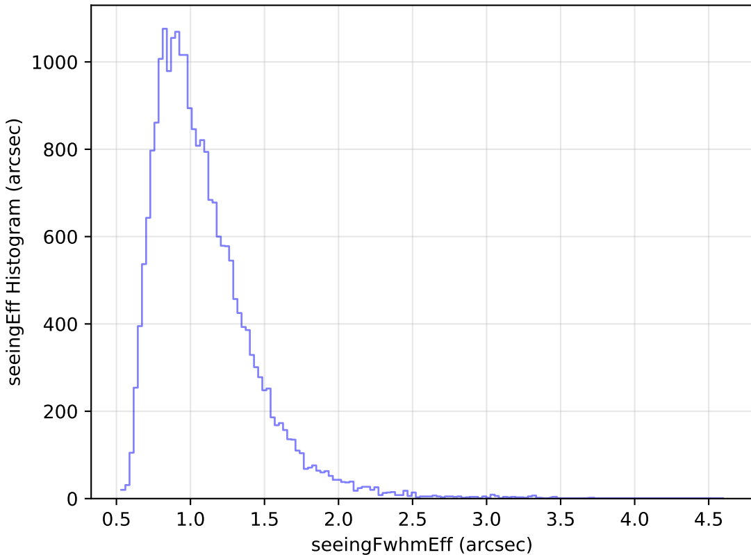
too_5_1v3.4_10yrs Yr 1 g band: seeingEff Histogram
