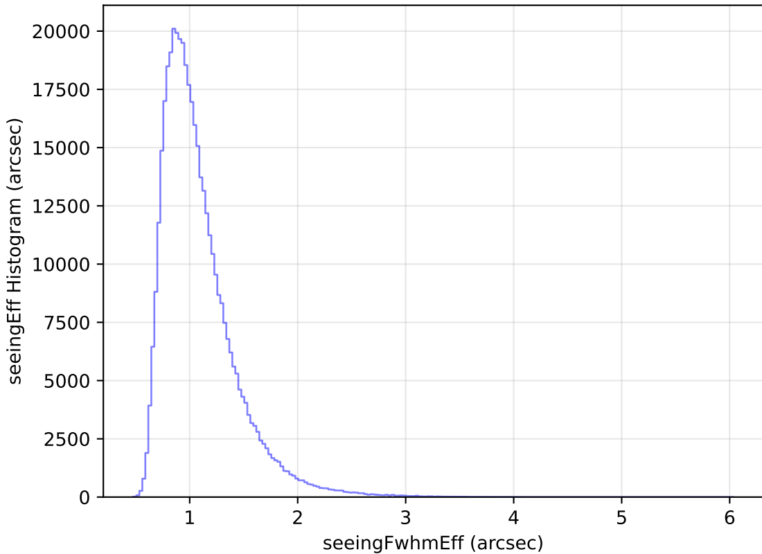
too_5_1v3.4_10yrs WFD z band: seeingEff Histogram
