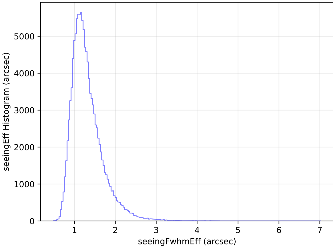
too_5_1v3.4_10yrs WFD u band: seeingEff Histogram
