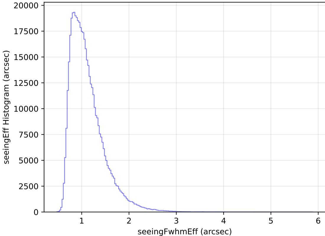
too_5_1v3.4_10yrs All sky r band: seeingEff Histogram
