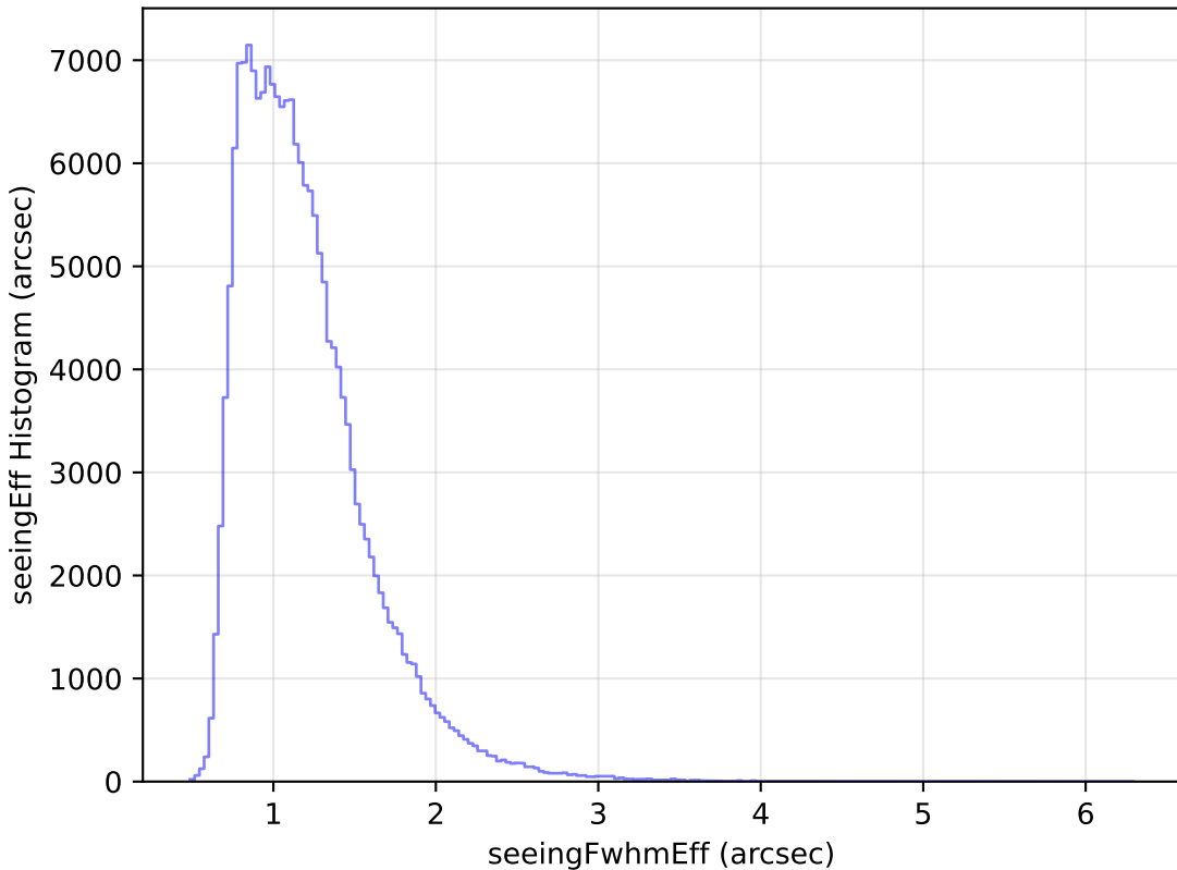
too_5_1v3.4_10yrs All sky g band: seeingEff Histogram
