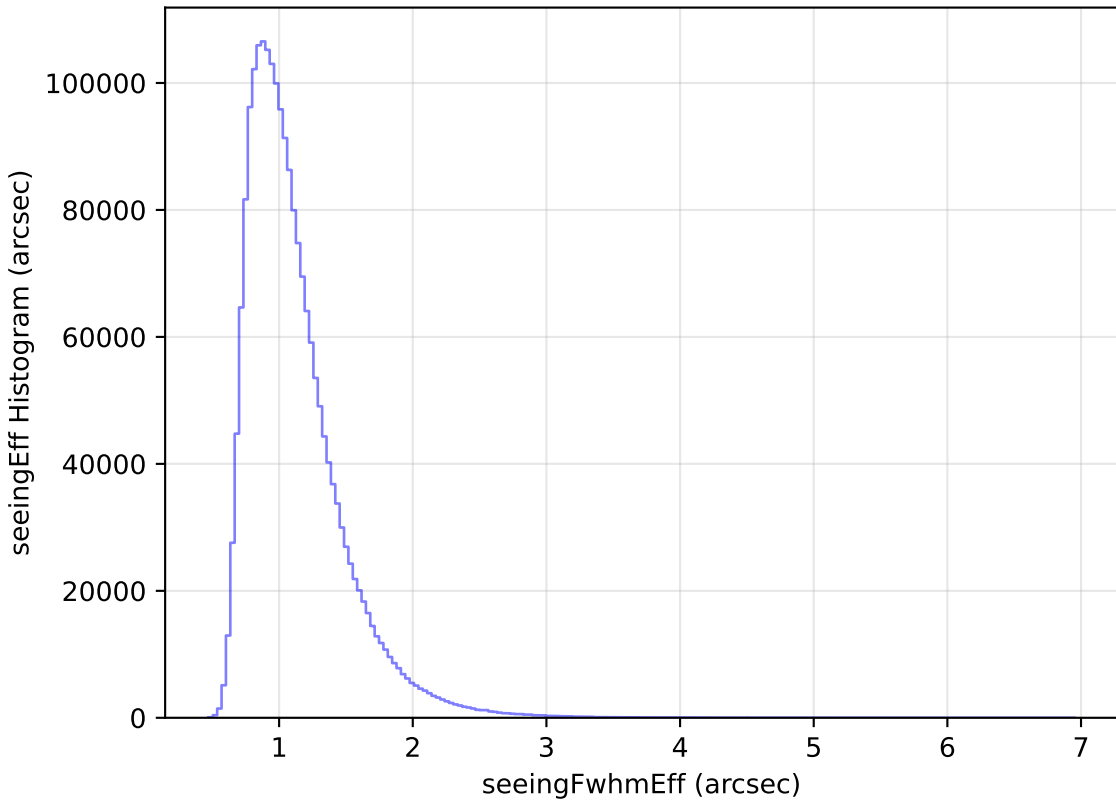
too_5_1v3.4_10yrs All sky all bands: seeingEff Histogram
