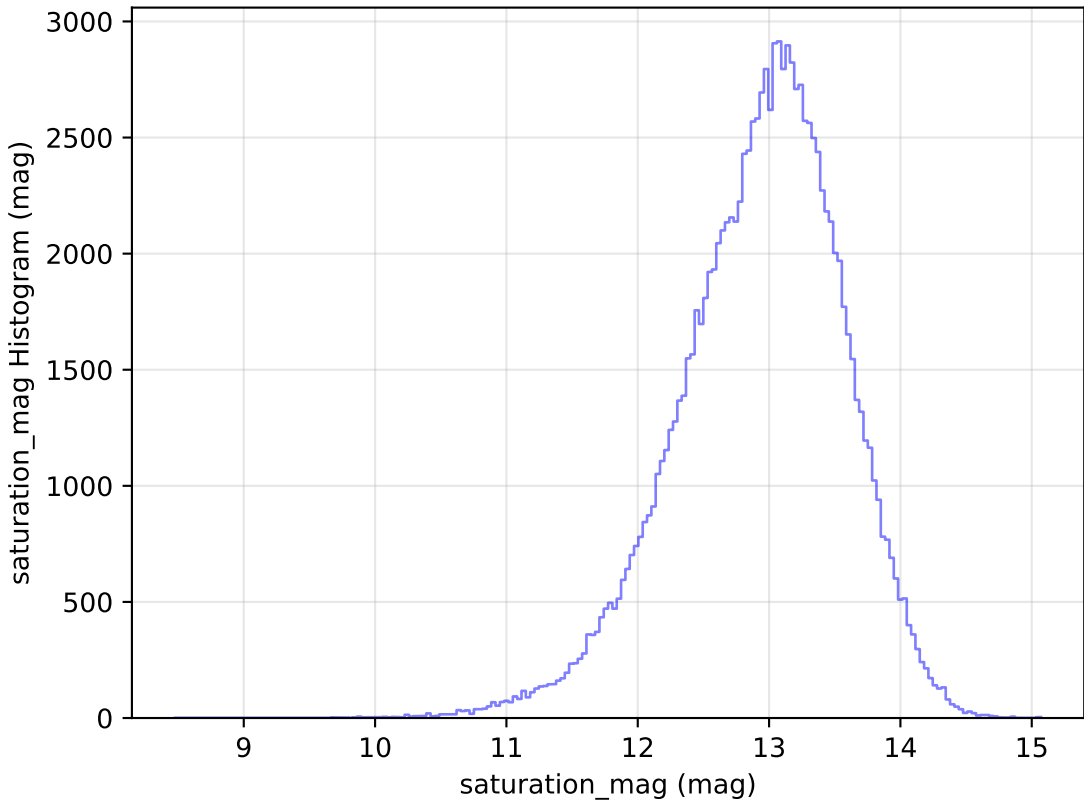
too_5_1v3.4_10yrs WFD u band: saturation_mag Histogram
