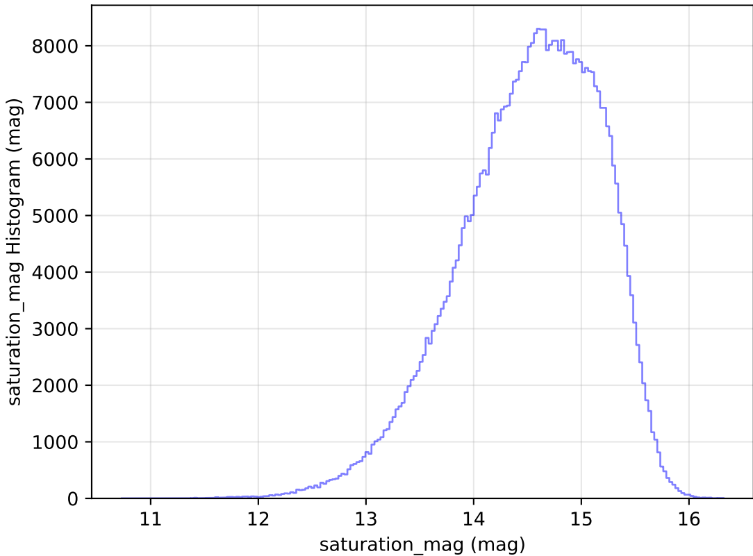
too_5_1v3.4_10yrs WFD r band: saturation_mag Histogram
