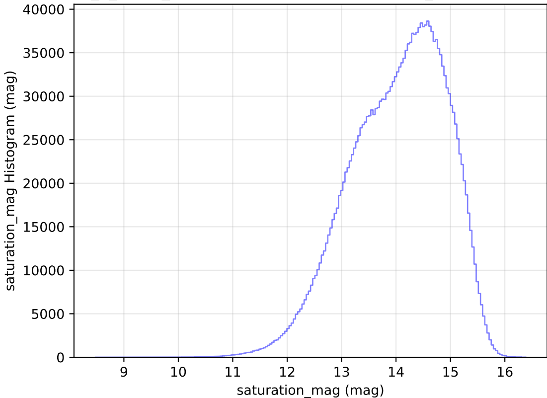
too_5_1v3.4_10yrs WFD all bands: saturation_mag Histogram
