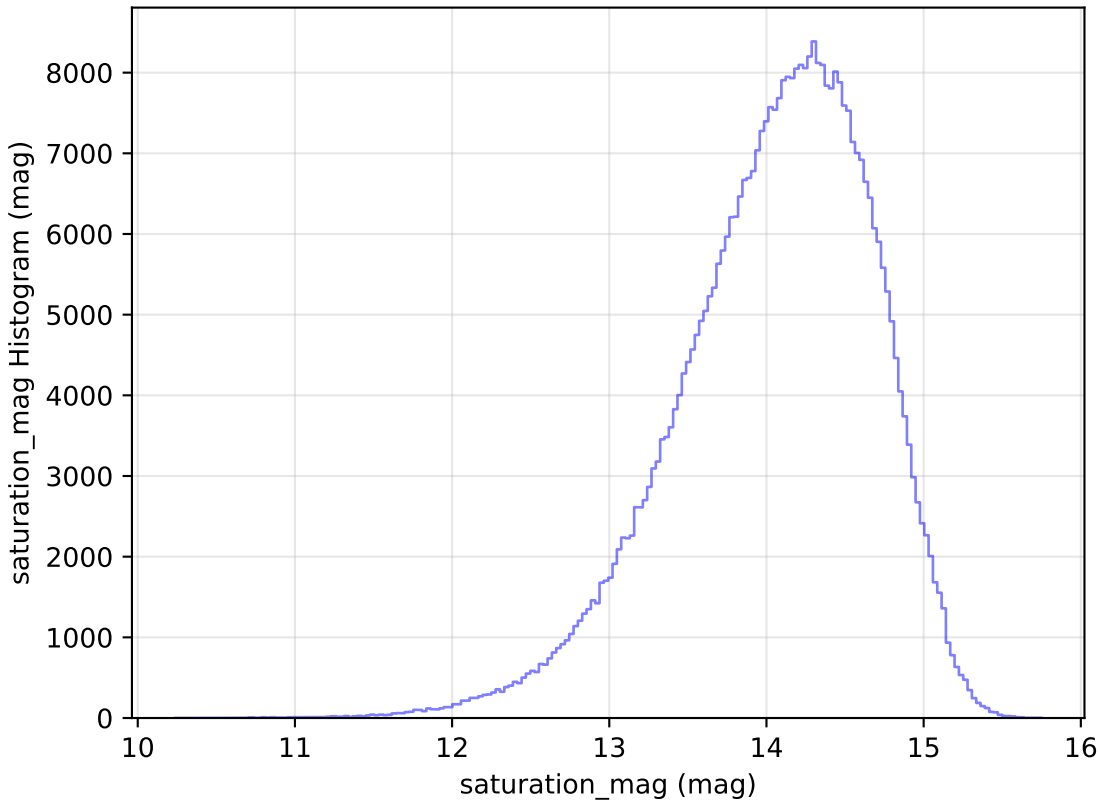
too_5_1v3.4_10yrs All sky z band: saturation_mag Histogram
