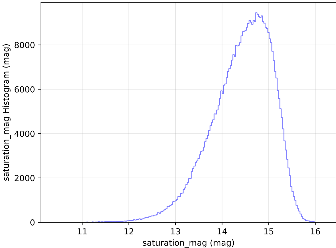
too_5_1v3.4_10yrs All sky i band: saturation_mag Histogram
