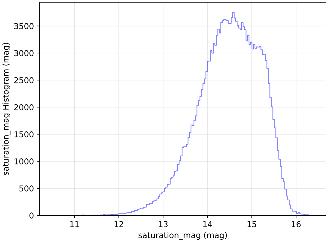
too_5_1v3.4_10yrs All sky g band: saturation_mag Histogram
