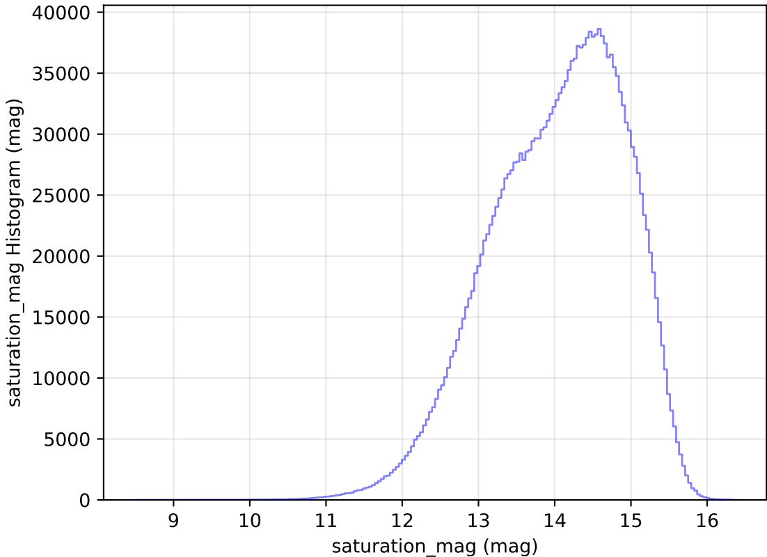
too_5_1v3.4_10yrs All sky all bands: saturation_mag Histogram
