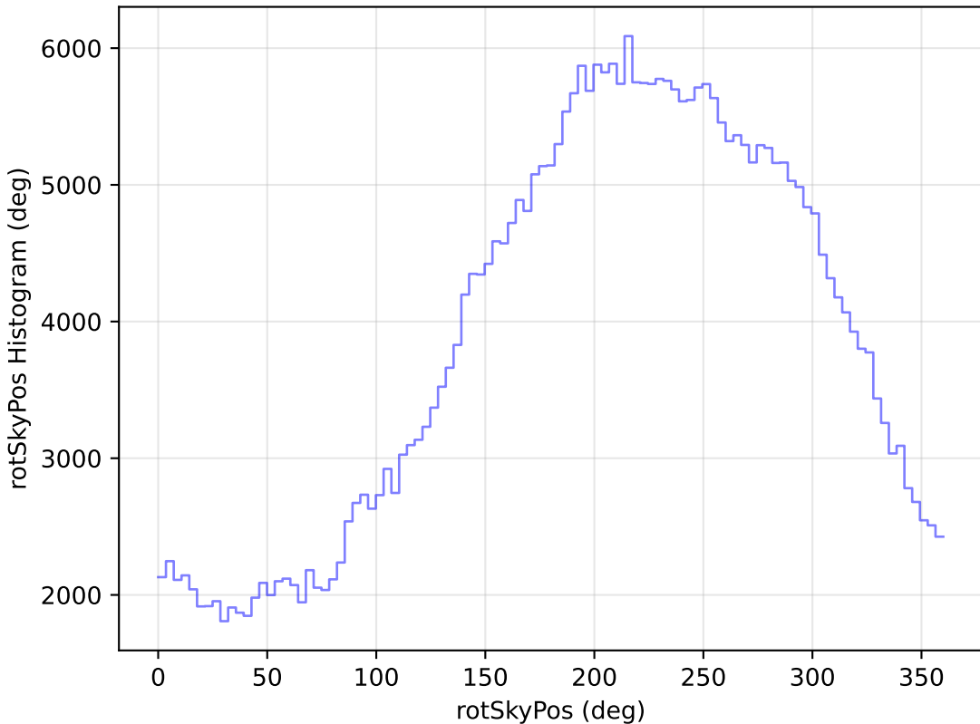
too_5_1v3.4_10yrs WFD y band: rotSkyPos Histogram
