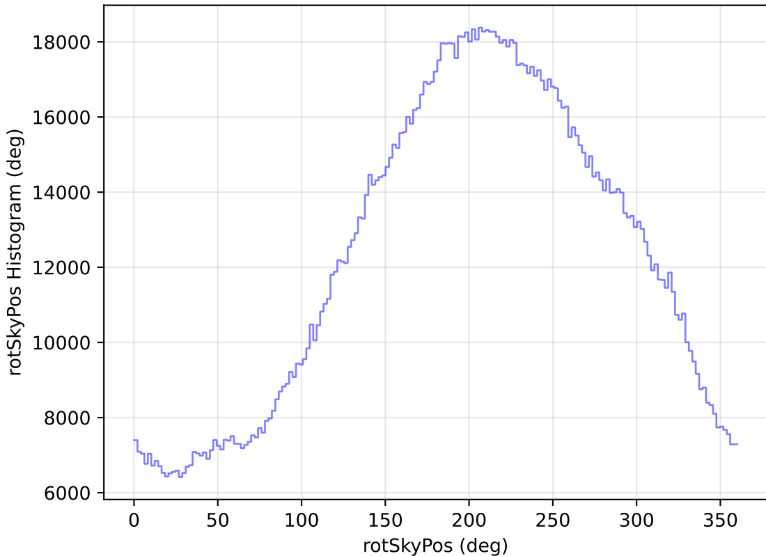
too_5_1v3.4_10yrs WFD all bands: rotSkyPos Histogram
