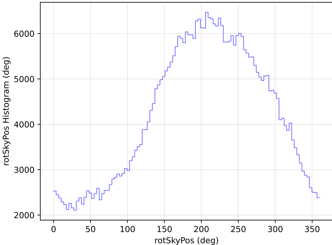
too_5_1v3.4_10yrs All sky z band: rotSkyPos Histogram
