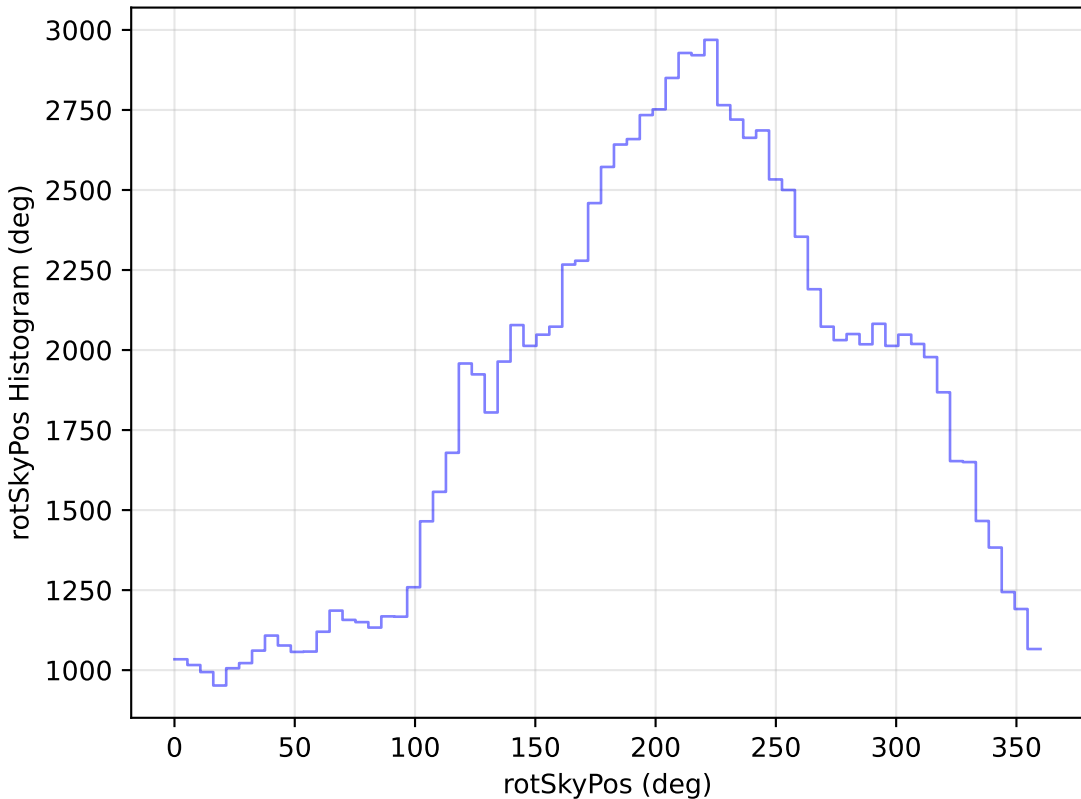
too_5_1v3.4_10yrs All sky u band: rotSkyPos Histogram
