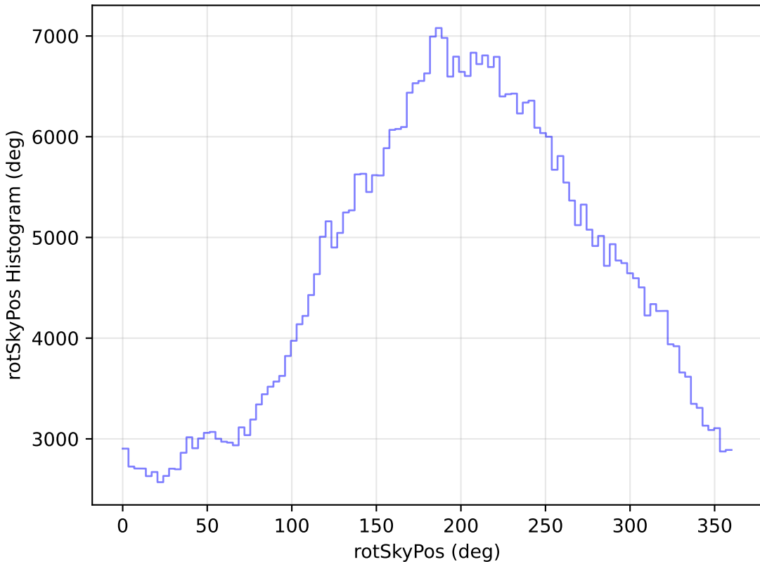
too_5_1v3.4_10yrs All sky r band: rotSkyPos Histogram
