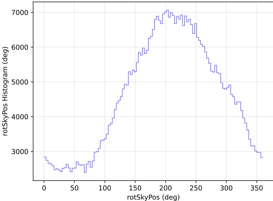
too_5_1v3.4_10yrs All sky i band: rotSkyPos Histogram
