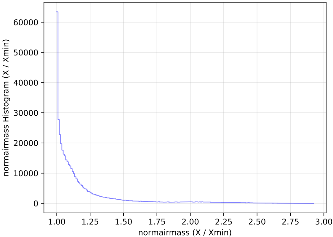
too_5_1v3.4_10yrs WFD z band: normairmass Histogram
