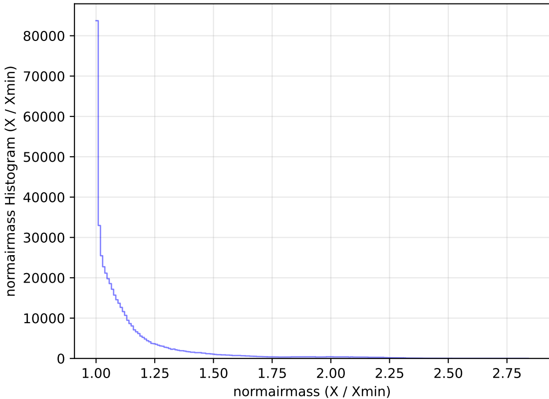
too_5_1v3.4_10yrs WFD r band: normairmass Histogram
